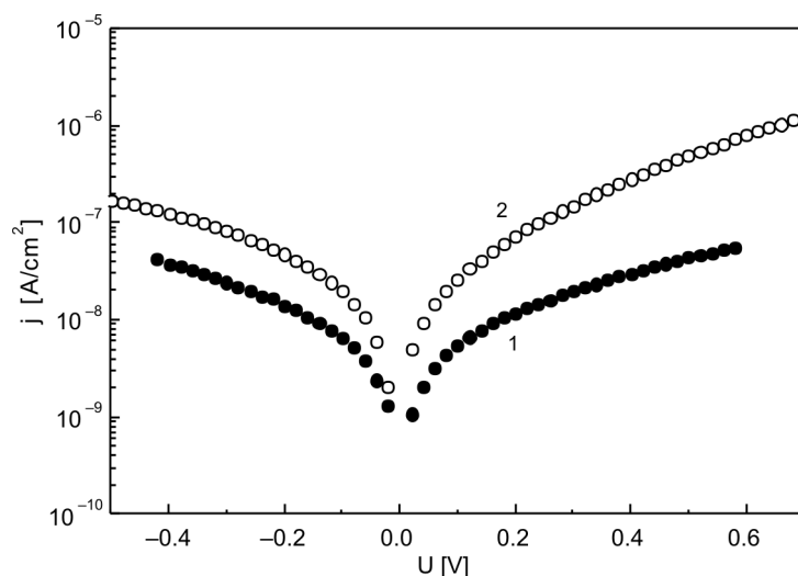
Fig. 3. Dark current-voltage curves of the investigated systems: 1 – \text{ITO}/\text{MoO}_3/\text{Tc}/\text{F}_{16}\text{ZnPc}/\text{Ag} , 2 – \text{ITO}/\text{MoO}_3/\text{Tc}/\text{F}_{16}\text{ZnPc}/\text{BCP}/\text{Ag} . Positive values of voltage refer to the higher potential on ITO
